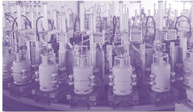
LPG Elektronical Carousel Refilling Cylinder
